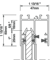
2-track | 2 carriles
