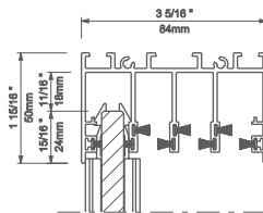
4-track | 4 carriles
