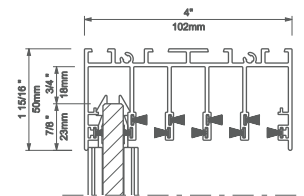
5-track | 5 carriles
