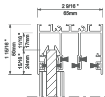
3-track | 3 carriles
